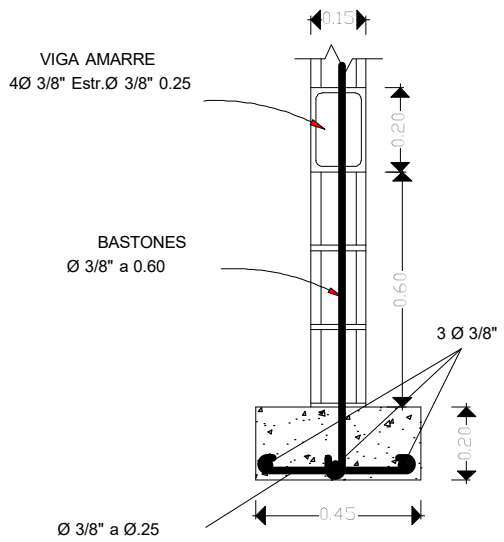
ZAPATA MURO 0.15 Mts.
